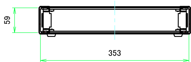
B-B ( 1:5.5 )
